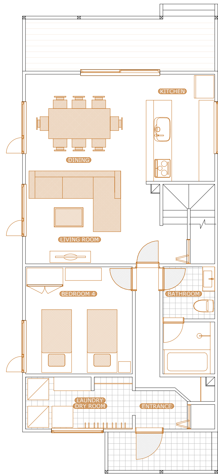
1st FLOOR
