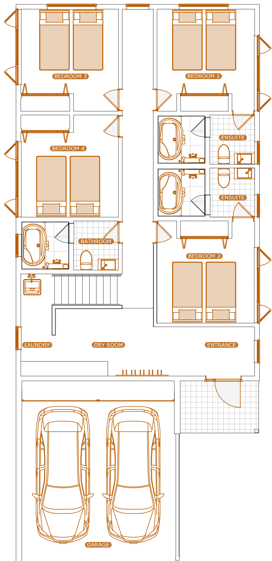
1st FLOOR
