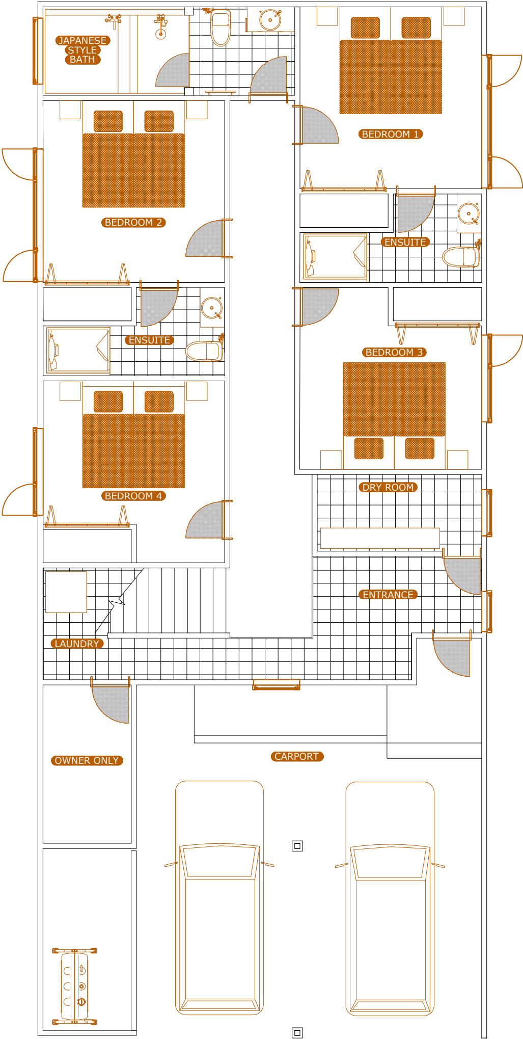
1st FLOOR
