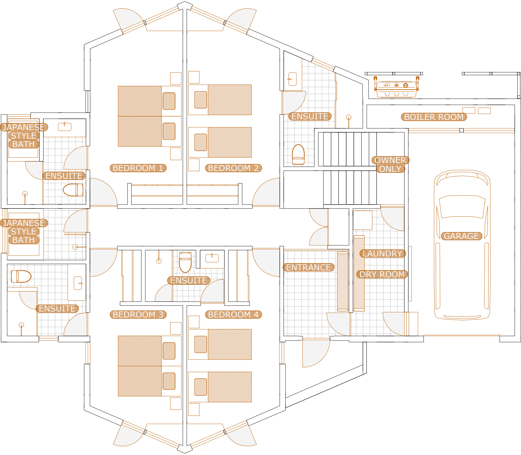
1st FLOOR
