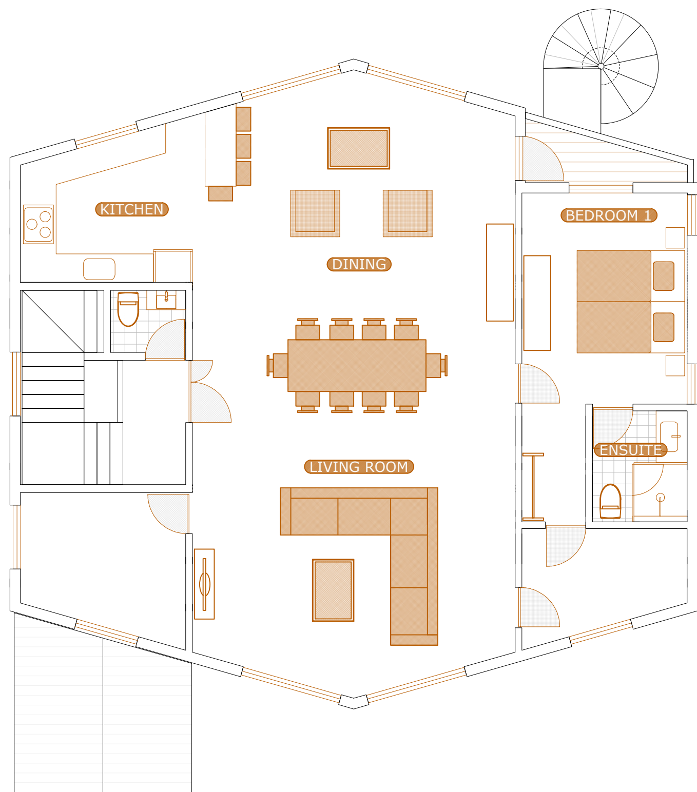
2nd FLOOR
