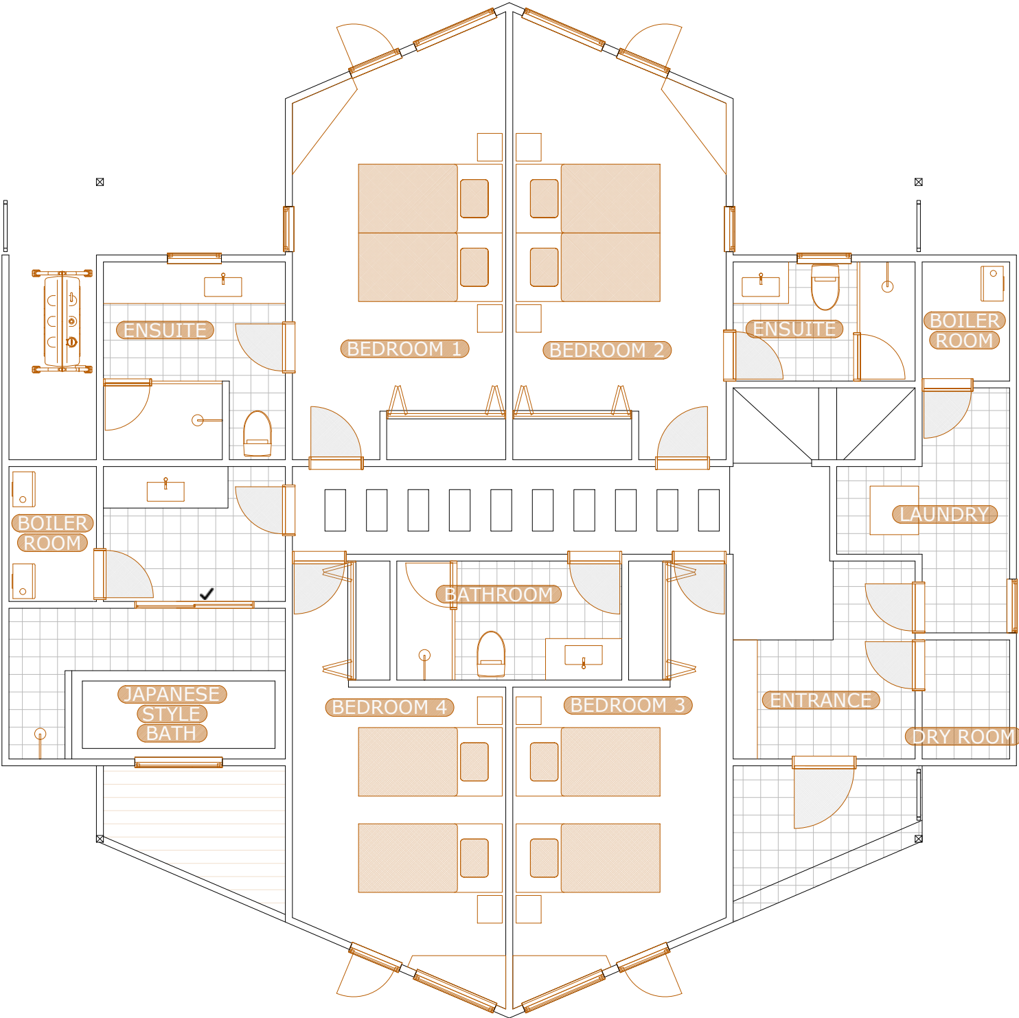
1st FLOOR
